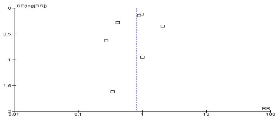
Figure 5: Publication Bias Using the Funnel Plot
